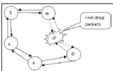
Fig 1: Jellyfish Attack
